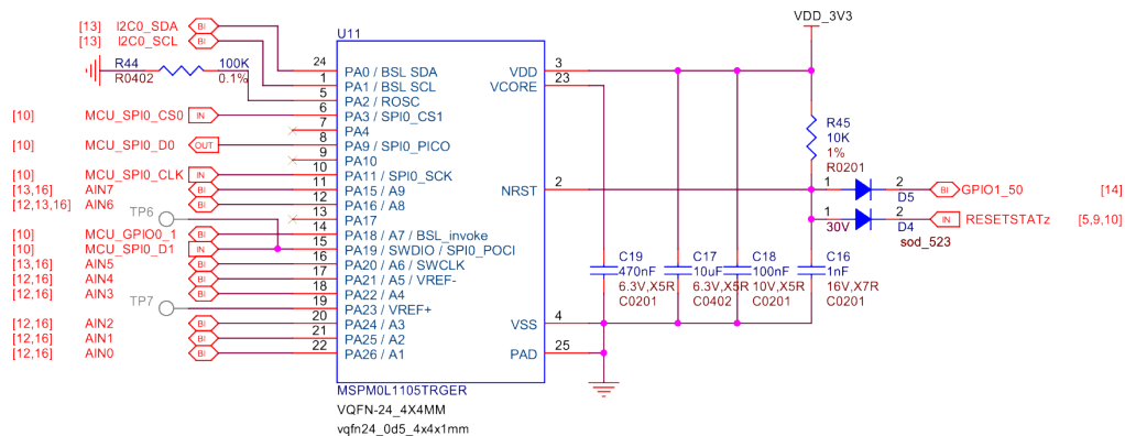
Fig. 3.41: MSPM0L1105 as 8ch 12bit ADC &amp; 4KB EEPROM
